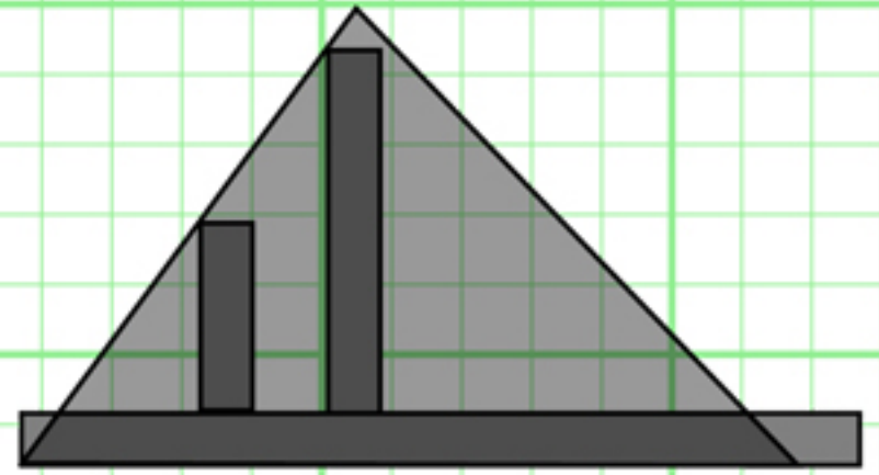
ALTERNATE SUPPORT BASE DETAIL (2X4 AND PLYWOOD)
